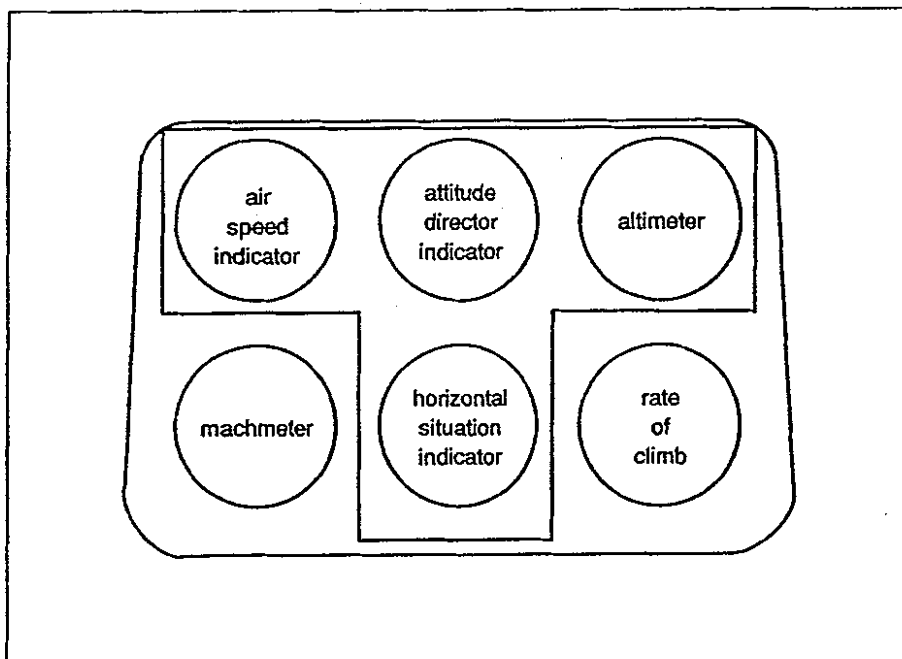
Figure 4-13. The "basic T panel" which forms the core of modern flight instrument panel layouts (adapted from Human Factors in Flight , F.H. Hawkins, 1987)
