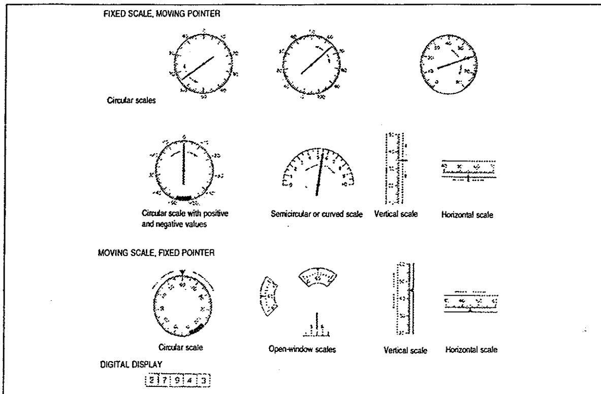
Figure 4-6. Example displays used in presenting quantitative information (adapted from McCormich et al. , 1983)
