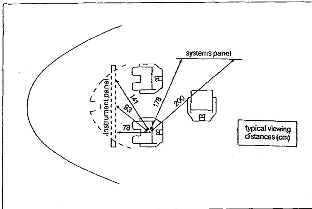
Figure 4-12. Typical viewing distances from the pilot's eye design eye position to various panels on the flight deck of a large jet (adapted from Human Factors in Flight , F.H. Hawkins, 1987)
