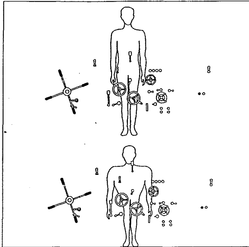
Figure 4-5. The controls of a lathe in current use are not within easy reach of the “average” person (from Applied Ergonomics IPC ; 1969; Vol. 1)
